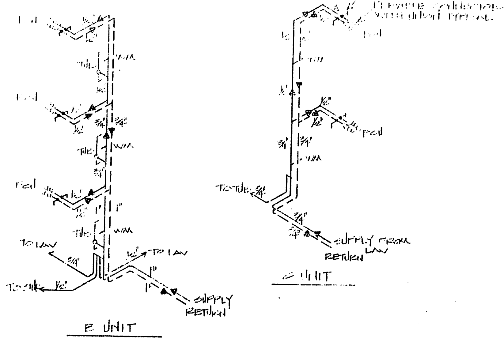
FAN COIL PIPING DETAILS
