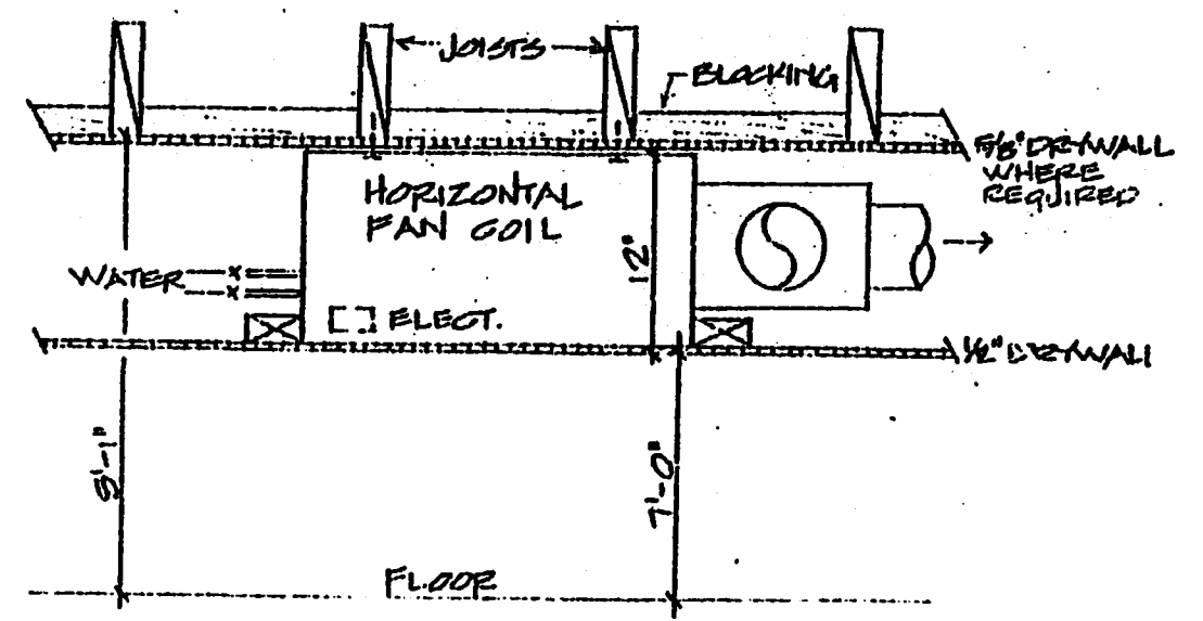
FAN COIL INSTALLATION DETAIL
